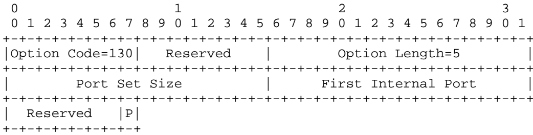
Figure 1: PORT_SET Option
