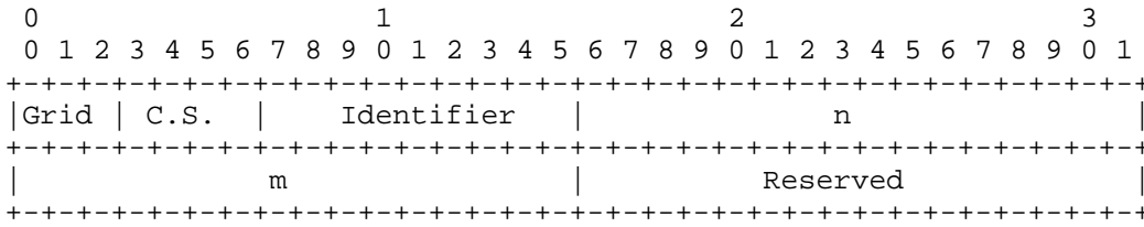
Figure 1 : The Flexi-Grid Label Encoding
