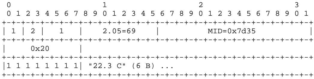
Figure 17: Confirmable Request; Piggybacked Response
