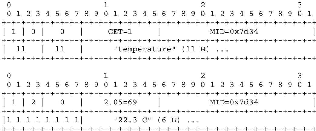
Figure 16: Confirmable Request; Piggybacked Response
