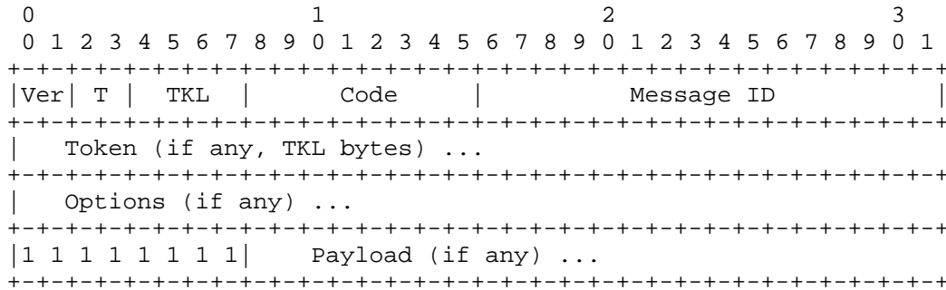
Figure 7: Message Format
