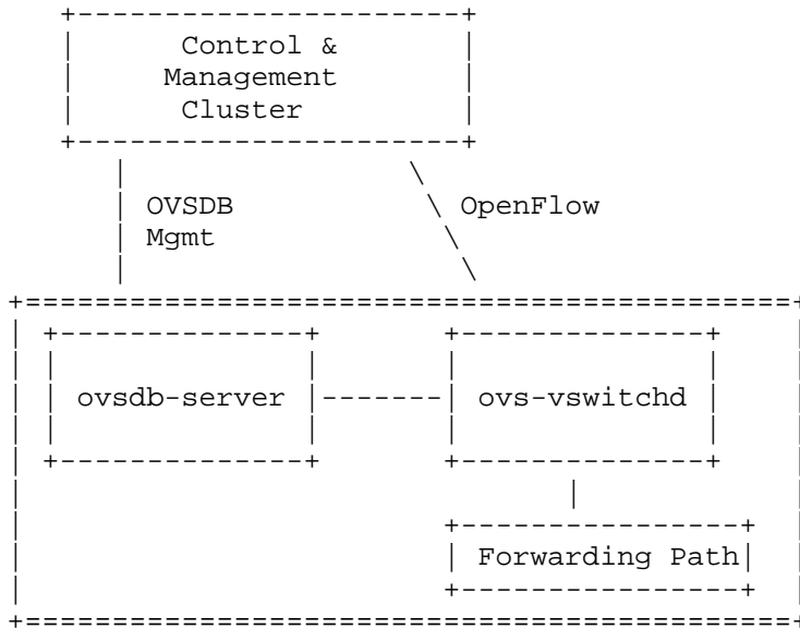
Figure 1: Open vSwitch Interfaces
