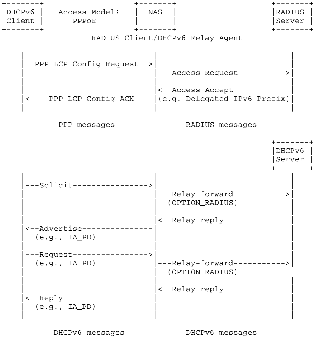
Figure 2: Network Scenario and Message Sequence When Employing DHCPv6 RADIUS Option in PPPoE Access
