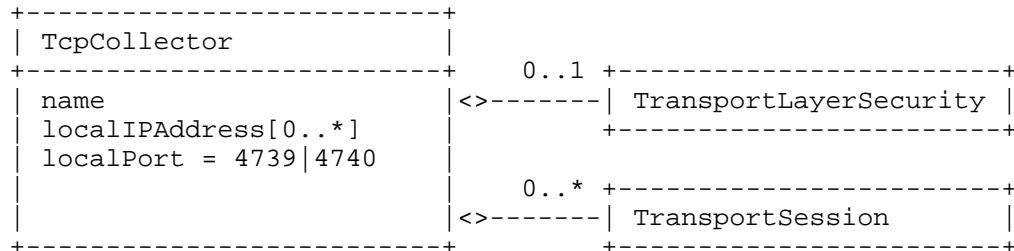
Figure 25: TcpCollector class
