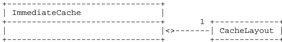
Figure 13: ImmediateCache class
