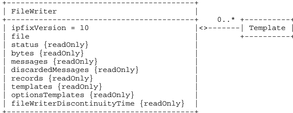
Figure 20: FileWriter classes
