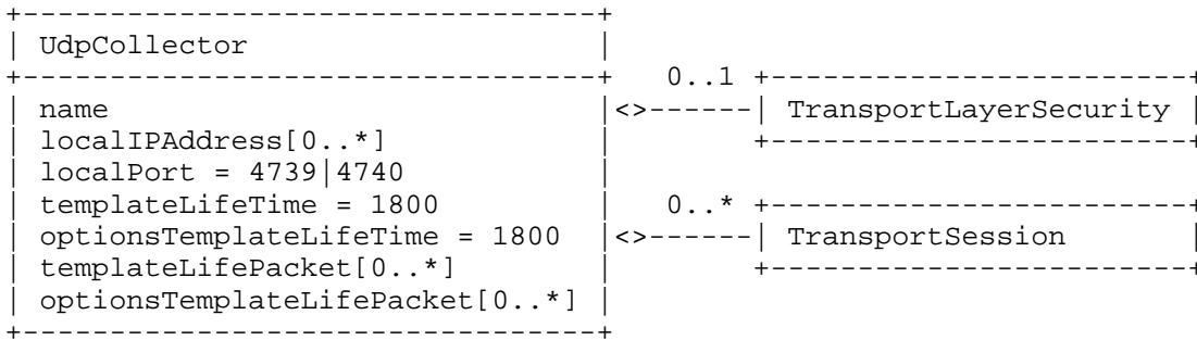
Figure 24: UdpCollector class
