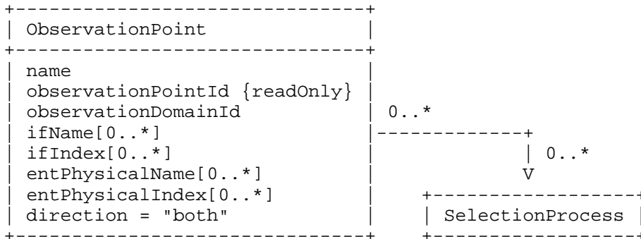
Figure 7: ObservationPoint class
