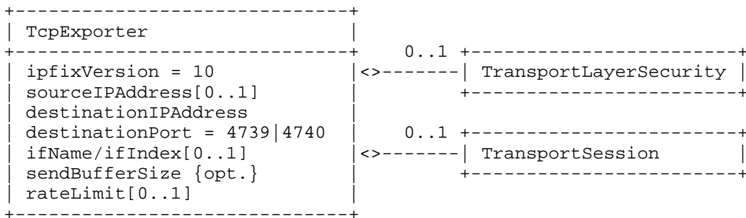
Figure 19: TcpExporter class
