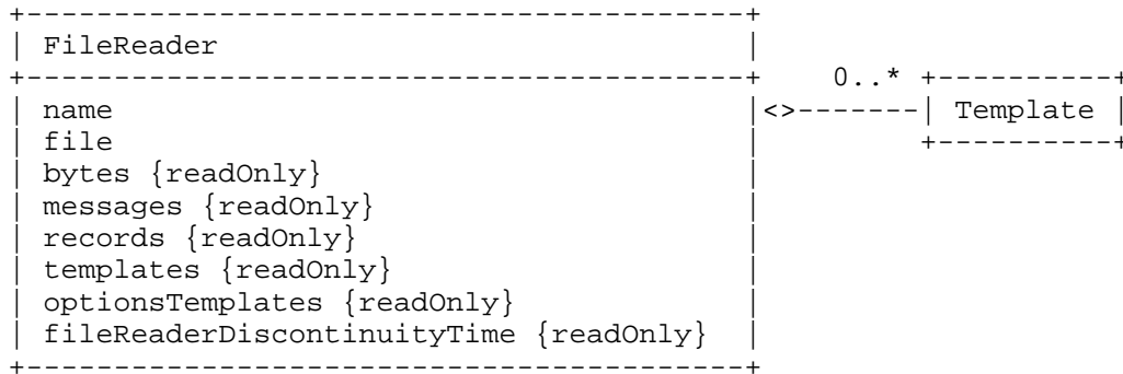
Figure 26: FileReader classes
