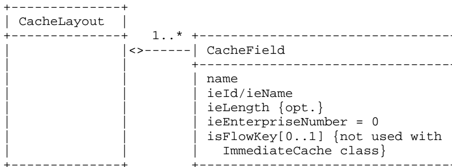
Figure 15: CacheLayout class
