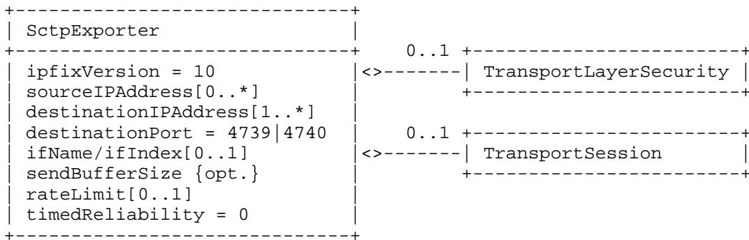
Figure 17: SctpExporter class
