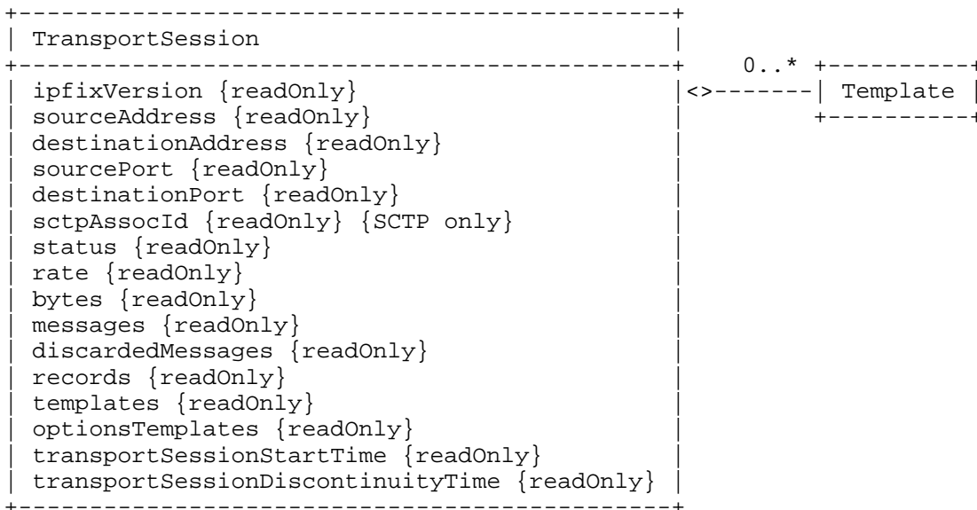
Figure 28: TransportSession class
