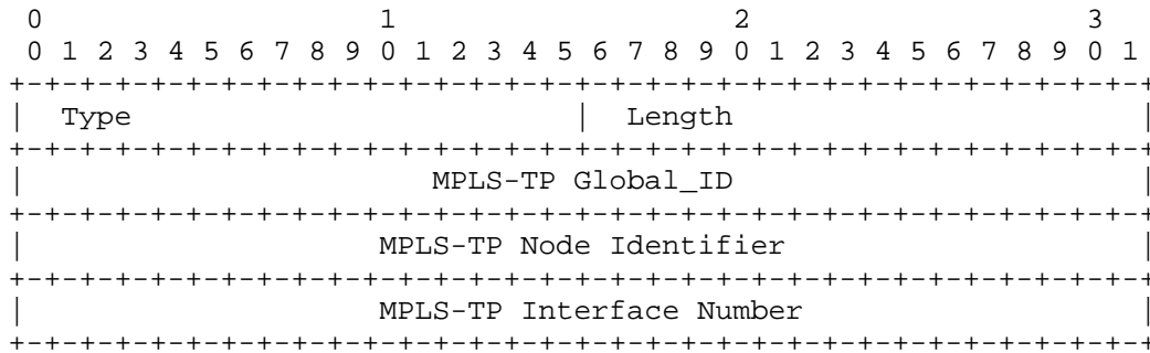
Figure 4: Section MEP-ID TLV Format
