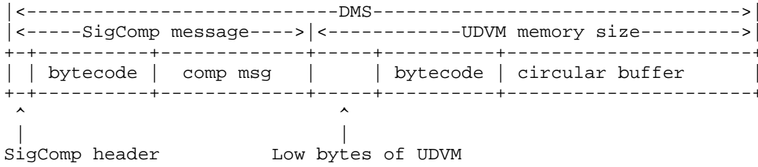
Figure 1: Bytecode and UDVM memory size within DMS
