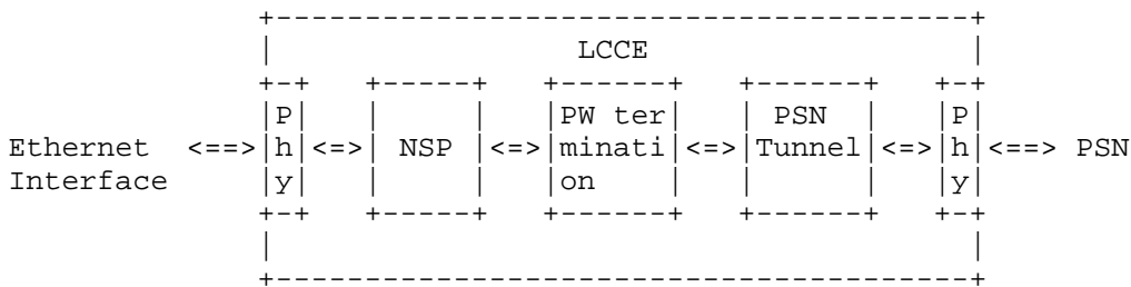
Figure 1: PW termination
