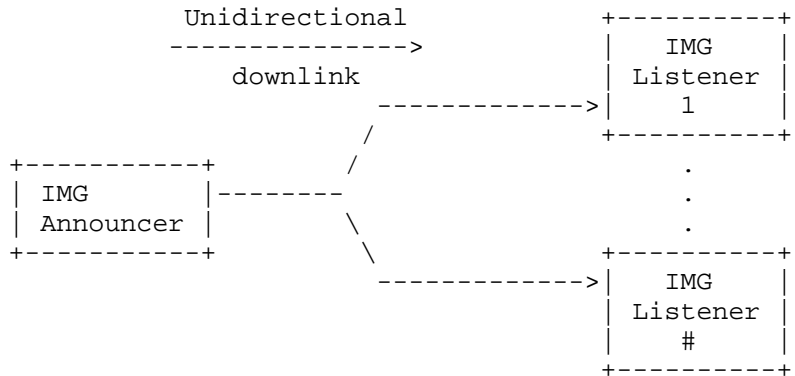
Figure 5: IMG Unidirectional Multicast Distribution Example
