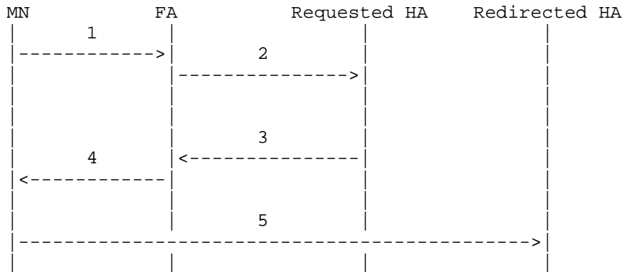
Figure 3: Example Message Flow for HA Redirection
