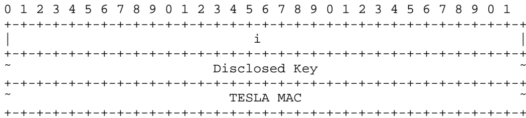
Figure 1. The "TESLA authentication extension".
