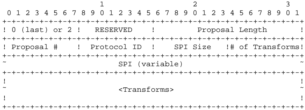
Figure 7: Proposal Substructure
