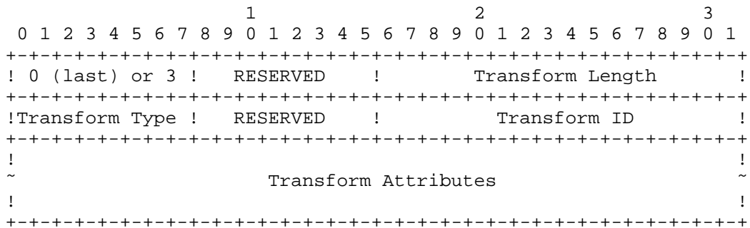
Figure 8: Transform Substructure
