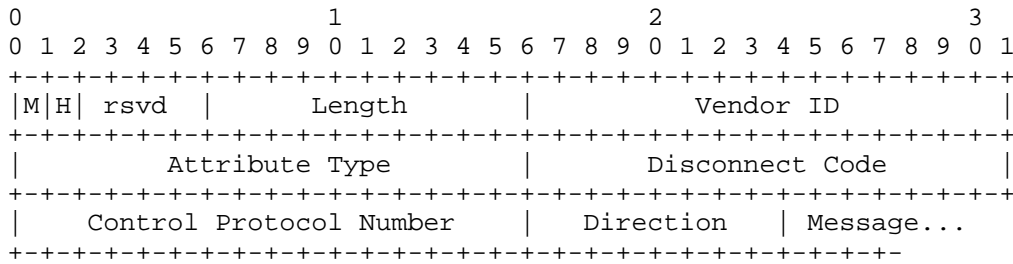
Figure 1: PPP Disconnect Cause Code AVP
