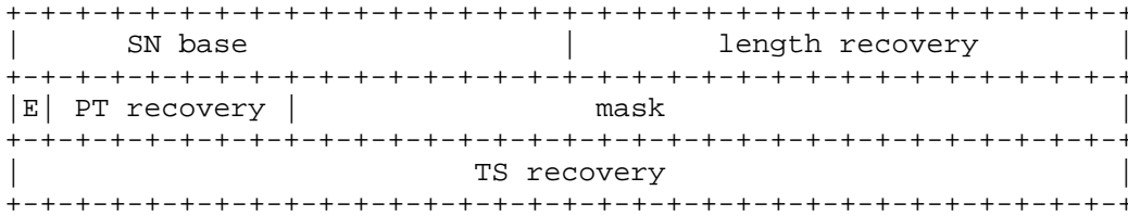
Figure 2: Parity Header Format
