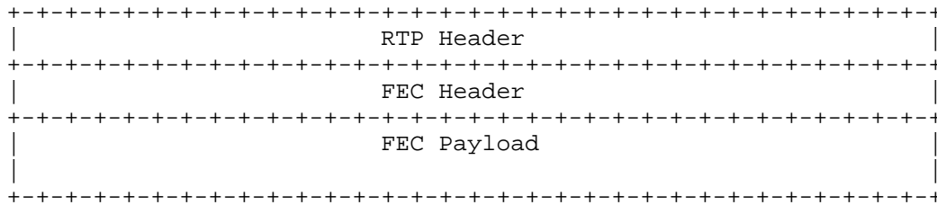
Figure 1: FEC Packet Structure
