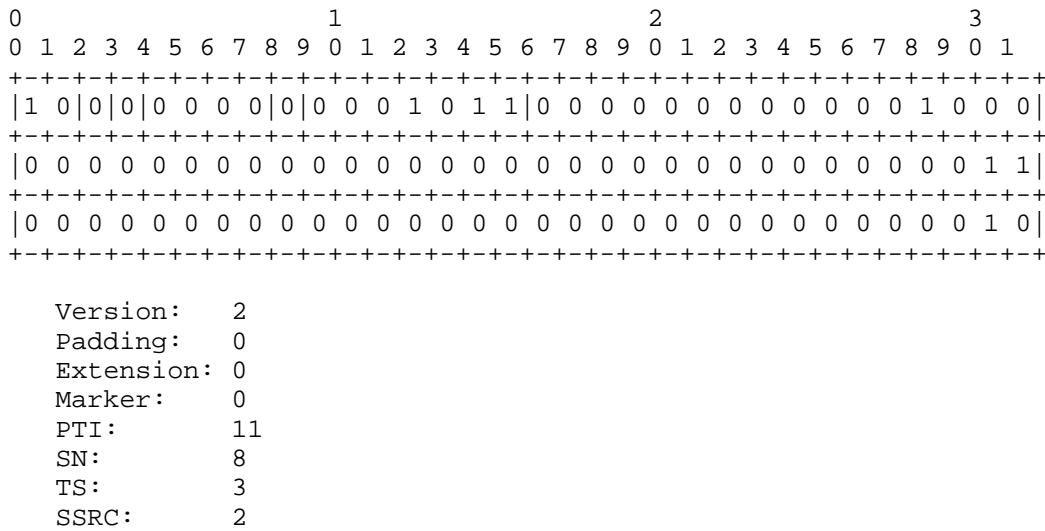
Figure 3: RTP Header for Media Packet X
