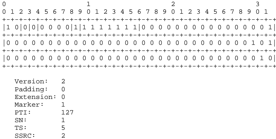
Figure 5: RTP Header of FEC for Packets X and Y
