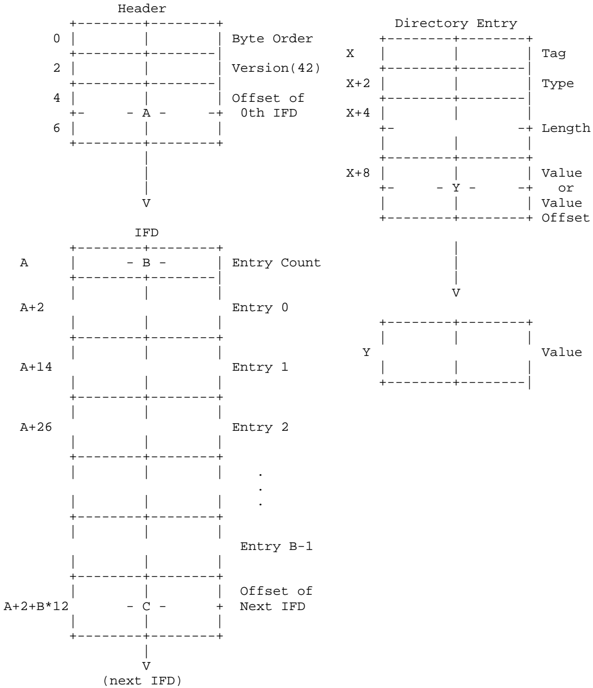
Figure 1: The Structure of a TIFF File
