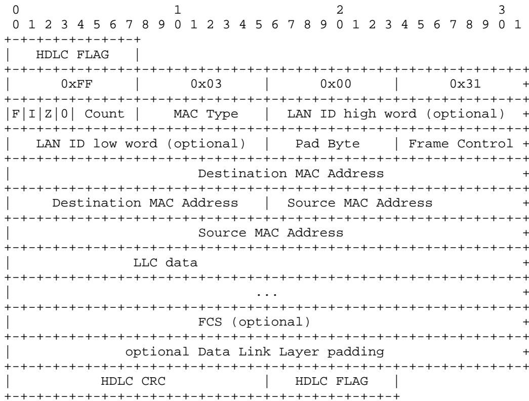
Figure 3: 802.4/802.5/FDDI Frame format
