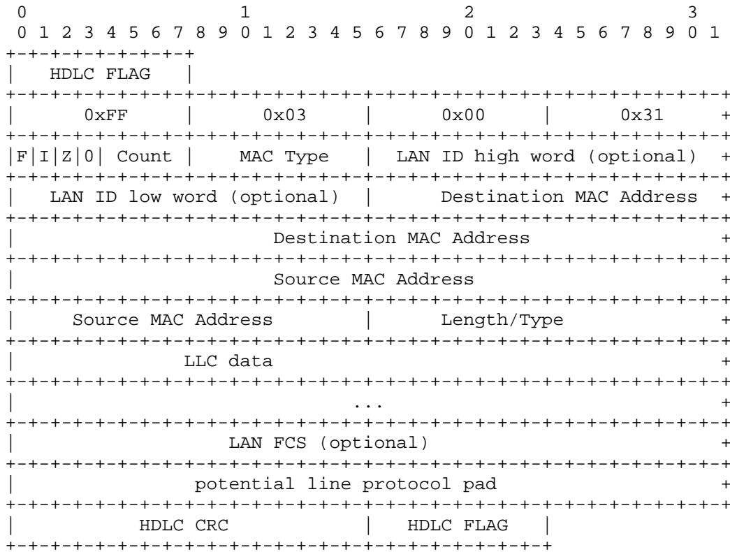
Figure 2: 802.3 Frame format
