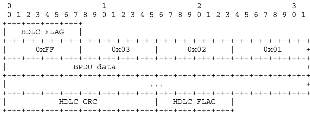
Figure 4: Bridge "Hello" PDU
