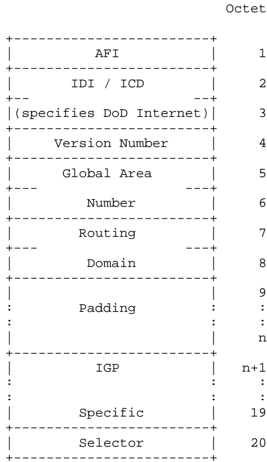
Figure 2: ISO IP address structure
