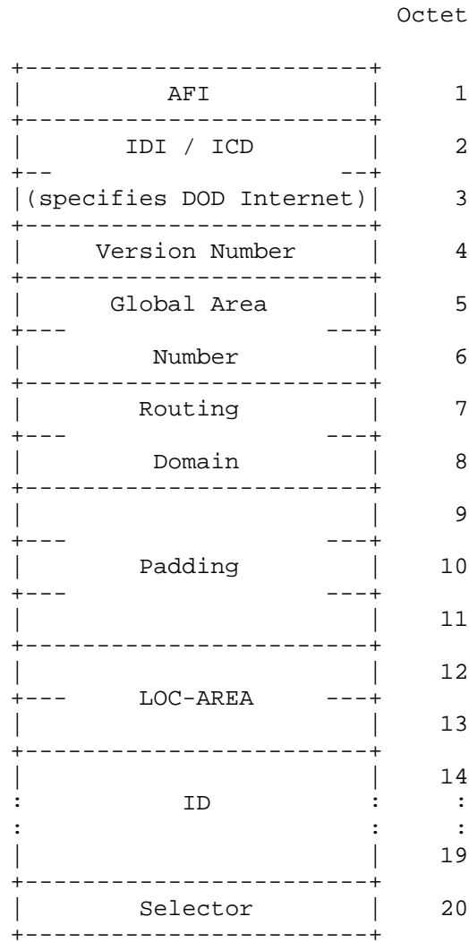
Figure 4: ISO IP Address with Encoded ANSI-format Address
