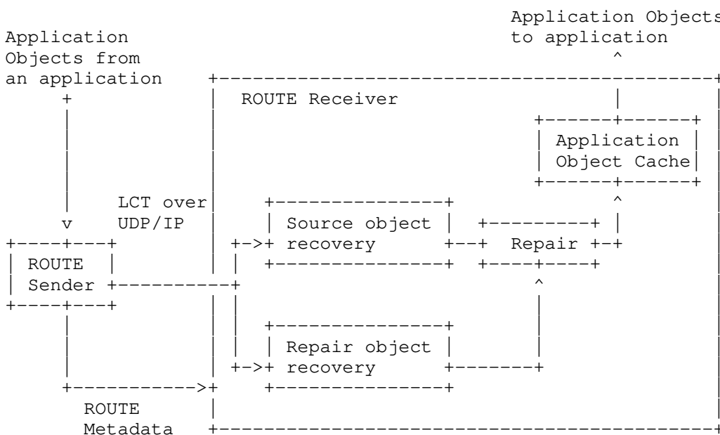
Figure 1: Architecture/Functional Block Diagram
