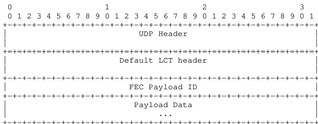
Figure 2: Overall ROUTE Packet Format
