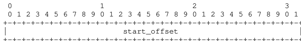
Figure 3: FEC Payload ID for Source Flows
