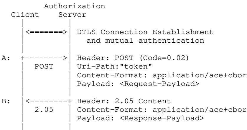
Figure 11: Token Request and Response Using Client Credentials
