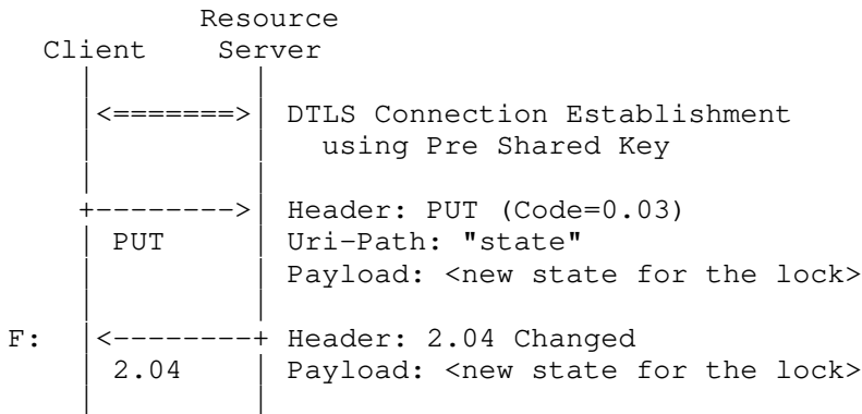
Figure 20: Resource Request and Response Protected by OSCORE
