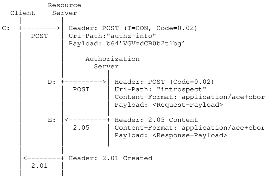
Figure 18: Token Introspection for the C Offline
