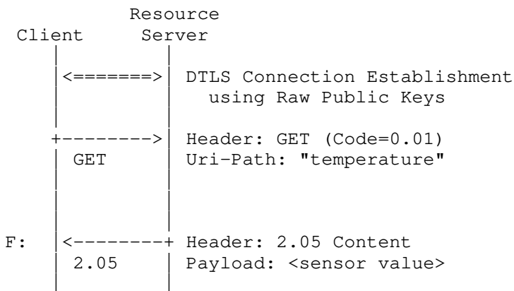
Figure 15: Resource Request and Response Protected by DTLS
