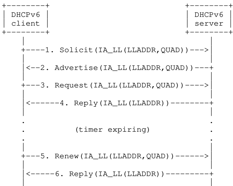
Figure 2: DHCPv6 Signaling Flow (Client-Server)
