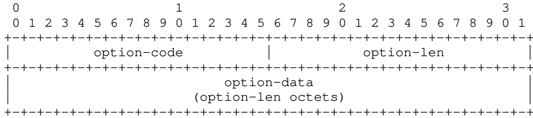
Figure 12: Option Format
