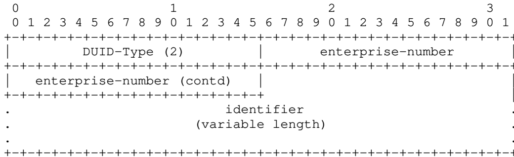
Figure 5: DUID-EN Format
