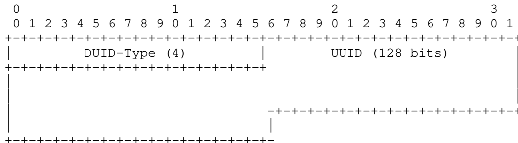
Figure 8: DUID-UUID Format
