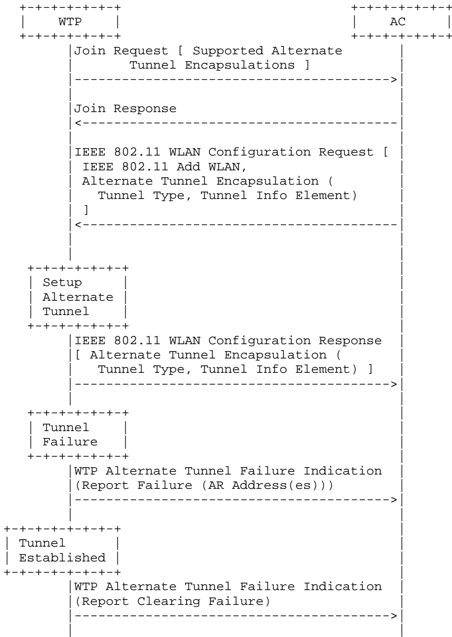
Figure 5: Setup of an Alternate Tunnel
