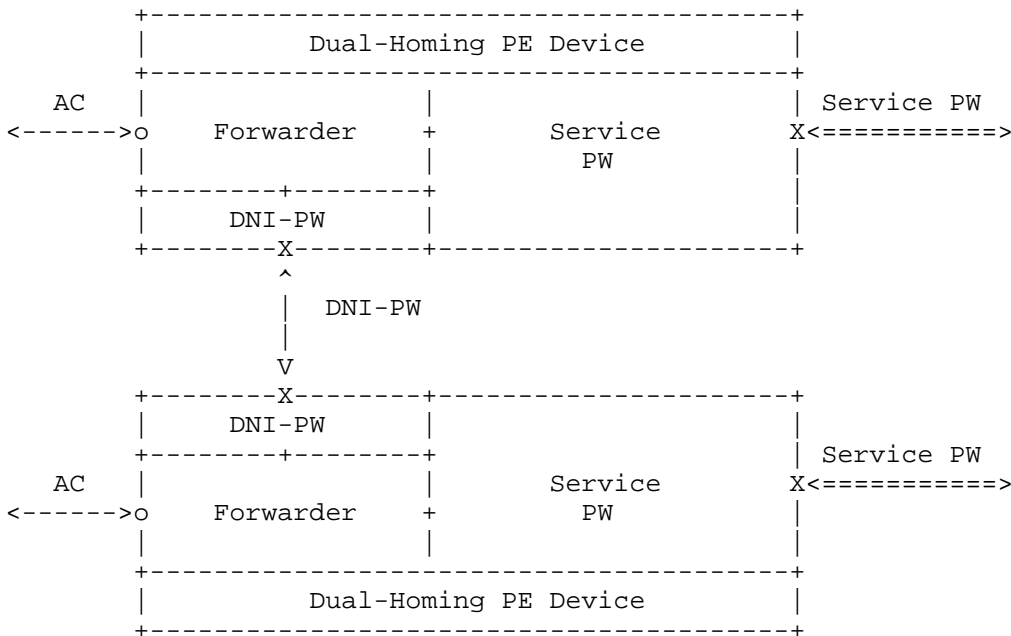
Figure 1: PE Architecture for Dual-Homing Protection
