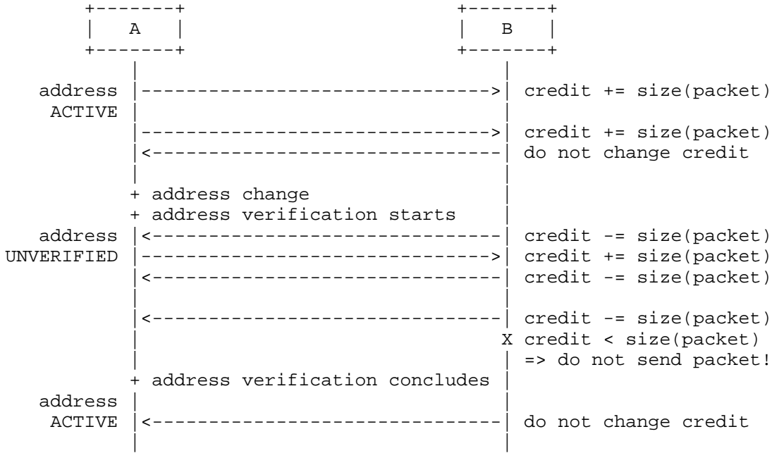
Figure 9: Readdressing Scenario
