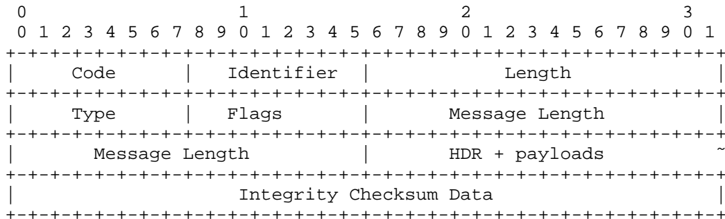
Figure 4: General Packet Format of EAP-IKEv2
