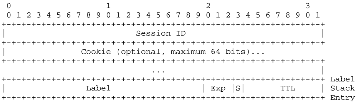
Figure 2.2 MPLS over L2TPv3 encapsulation
