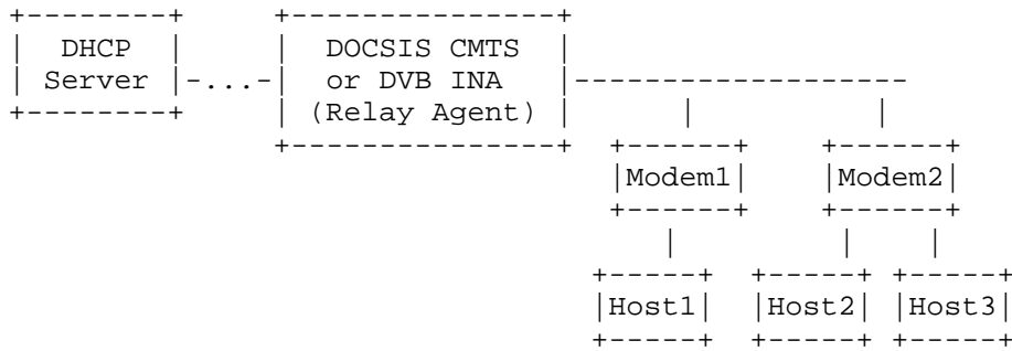
Figure 1: Cable Environment for DHCPLEASEQUERY
