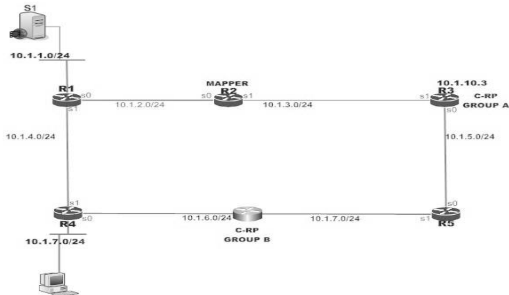
Figure 25 network design with one multicast domain
