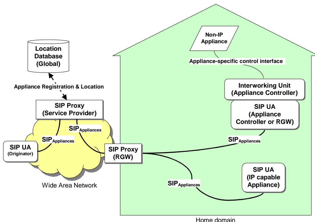
Figure 4: Example Functional Architecture for Remote Communication with Networked Appliances
