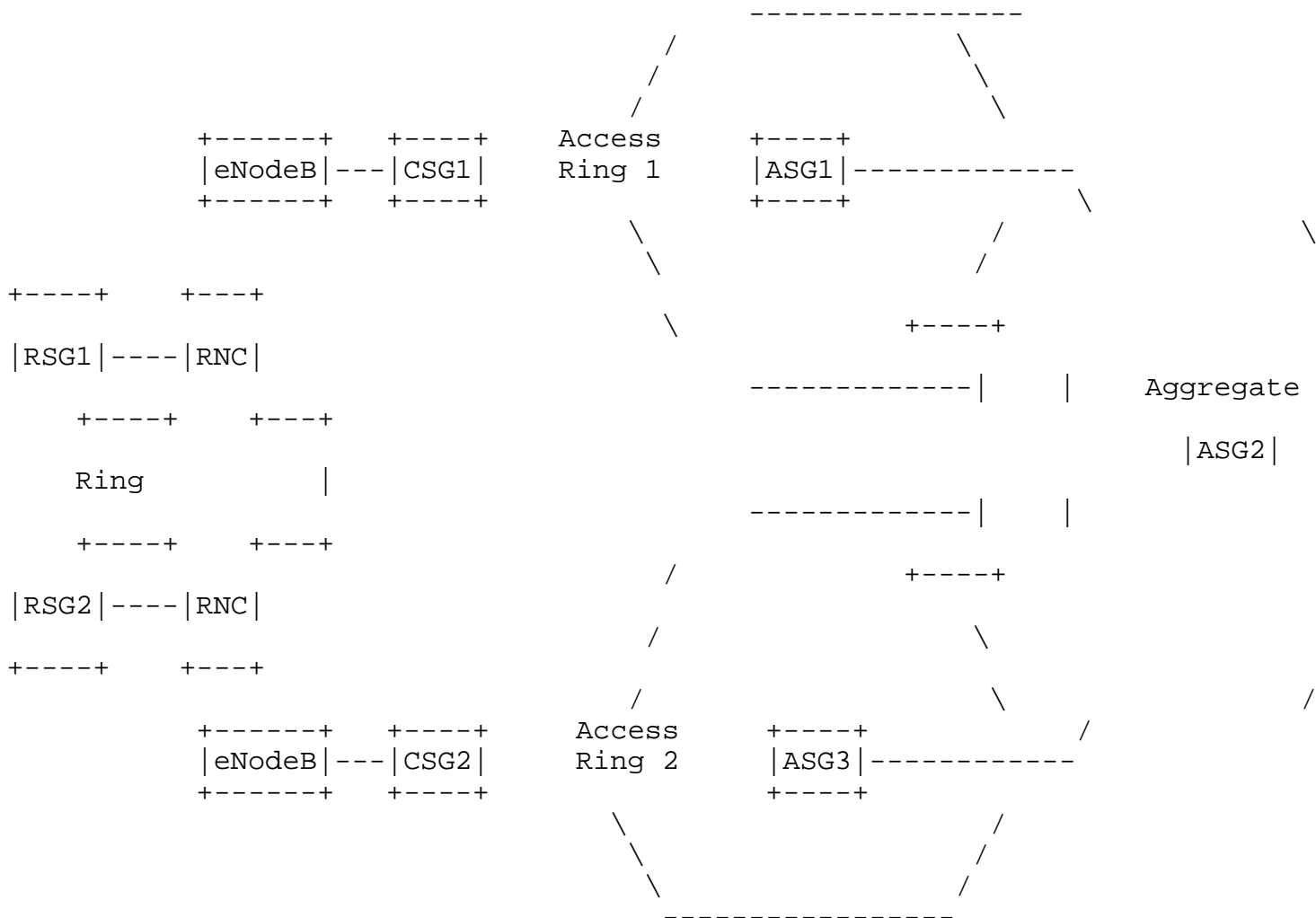
Figure 2: Mobile Backhaul Network
