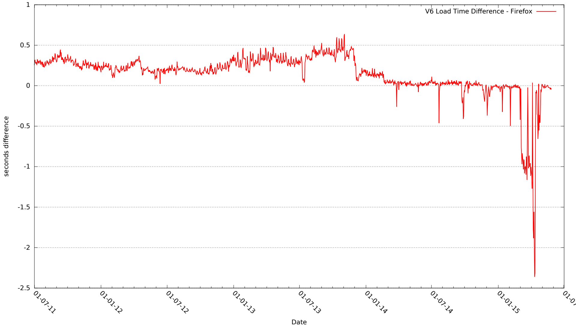
Avg V6 Load Time Differential (secs) - Firefox
