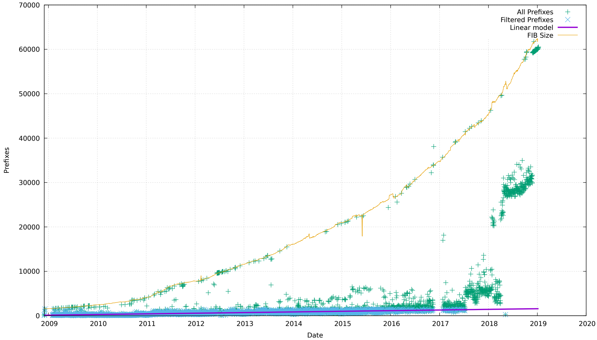
BGP v6 Daily Unstable Prefix Count
