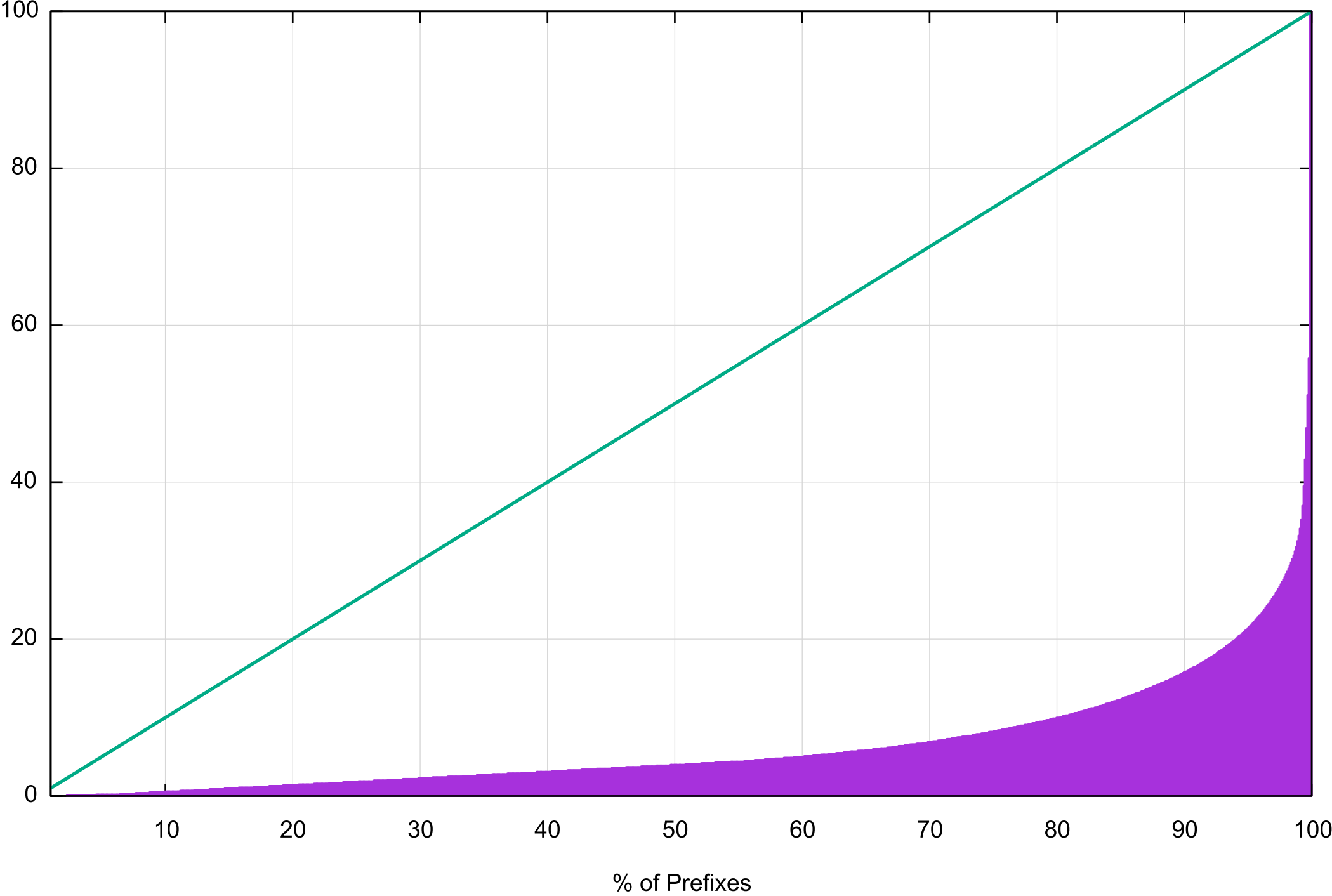
BGP Prefix Update Cumulative Distribution
