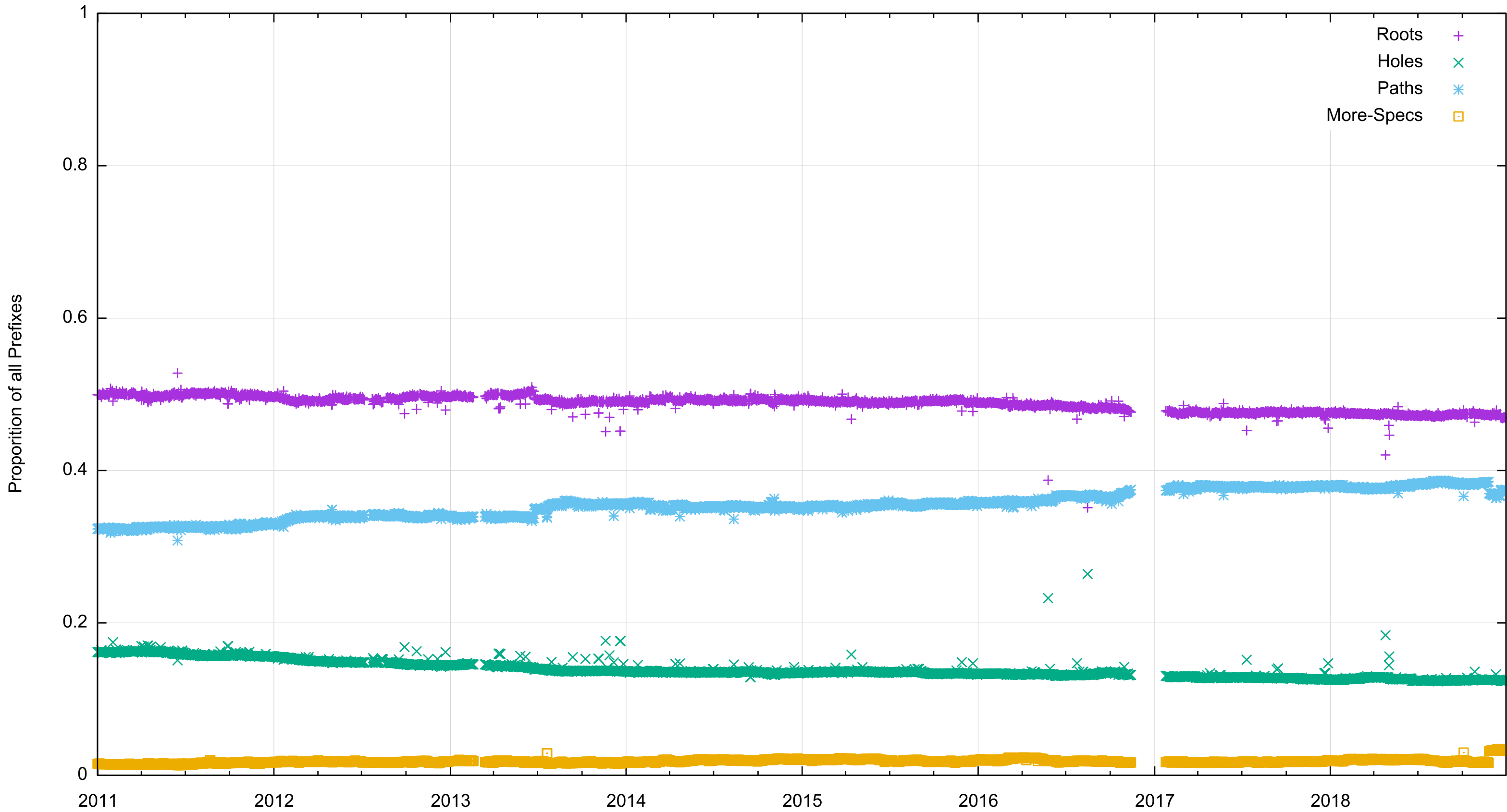
Prefix Types - IPv6
