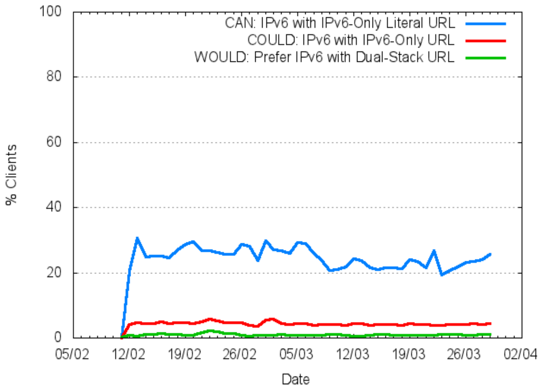
Client IPv6 Capability by URL Type (***)
