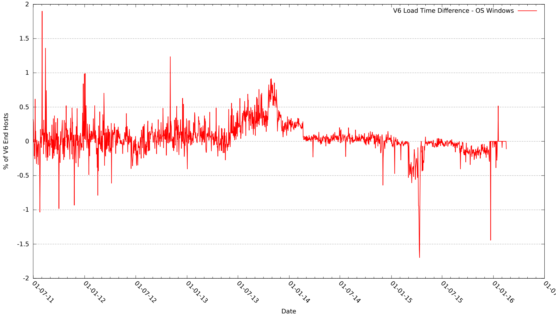
Avg V6 Load Time Differential (secs) - OS Windows
