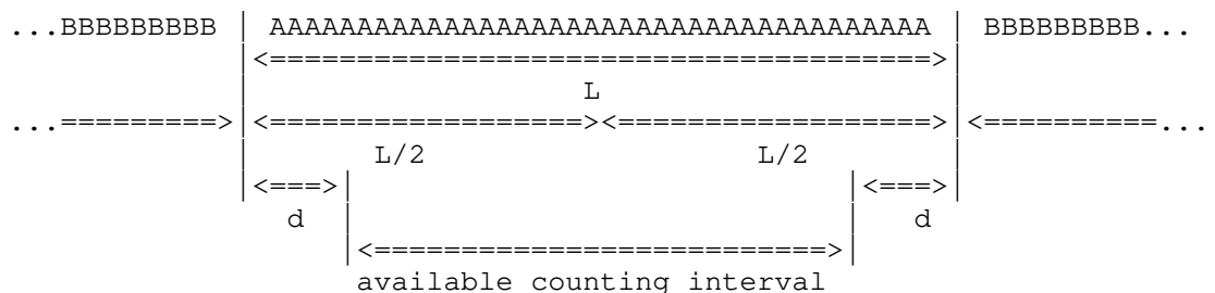
Figure 4: Timing Aspects
