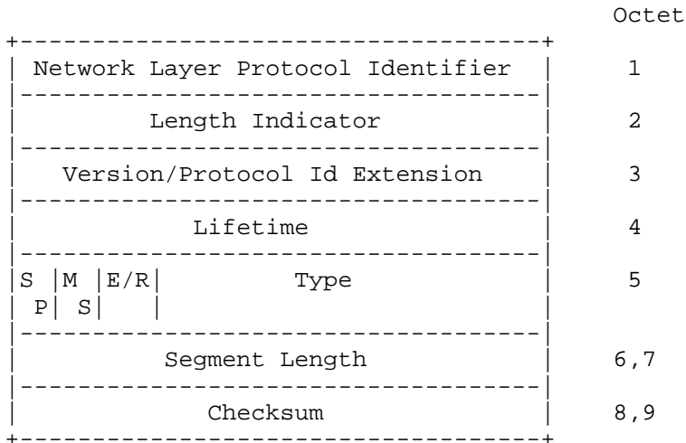
Figure 7-2. PDU Header--Fixed Part
