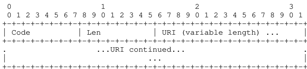
Figure 1: Captive-Portal DHCPv4 Option Format
