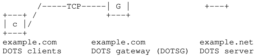
Figure 6: Client-Side Gateway with Aggregation
