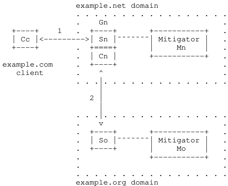
Figure 12: Recursive Signaling
