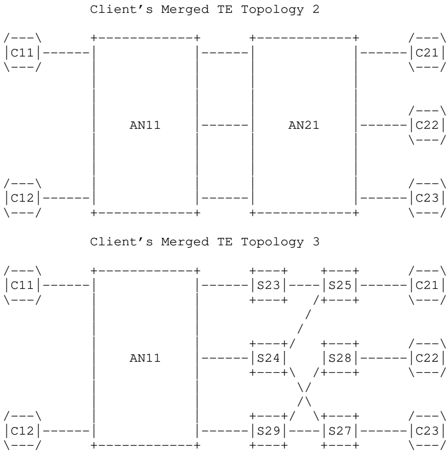
Figure 15: Multiple Native (Merged) Client's TE Topologies
