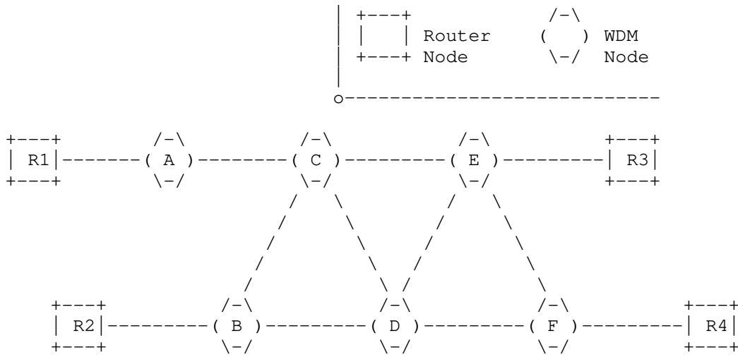
Figure 9: Example Packet Optical Topology
