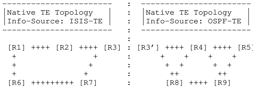
Figure 8: Native TE Topologies as Seen on Node R3
