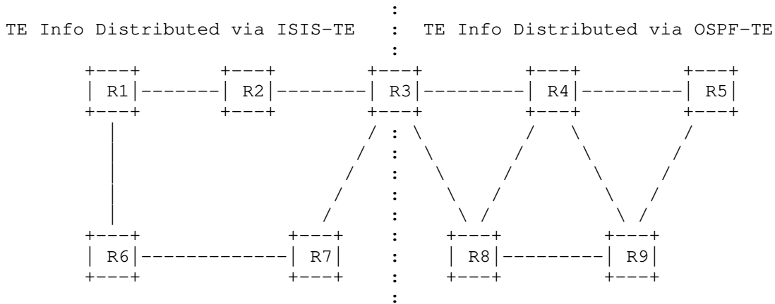
Figure 7: Example Split Network Topology
