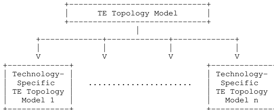
Figure 17: Augmenting the Technology-Agnostic TE Topology Model
