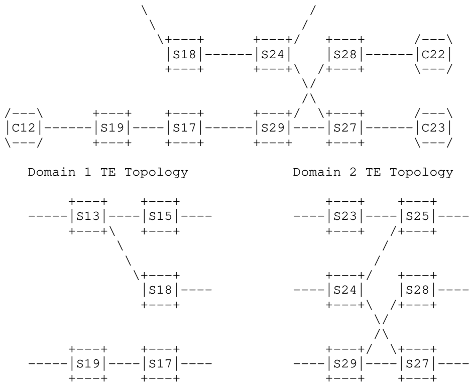
Figure 13: Merging Domain TE Topologies: An Example
