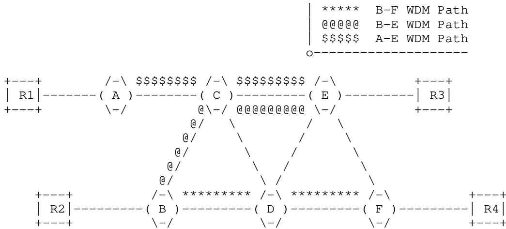
Figure 10: Paths within the Provider Domain
