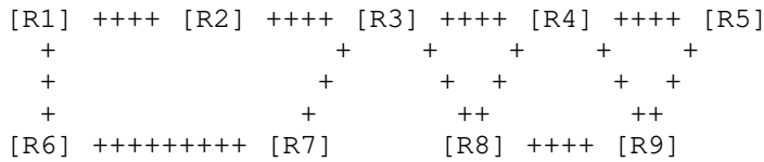
Figure 6: Native TE Topology as Seen on Node R3
