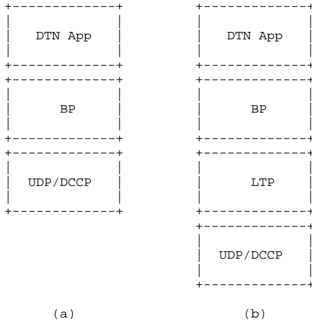
Figure 2: Protocol Stacks Addressed in this Document
