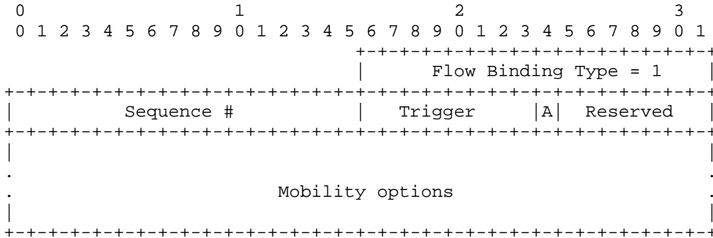
Figure 3: Flow Binding Indication Mobility Header Format
