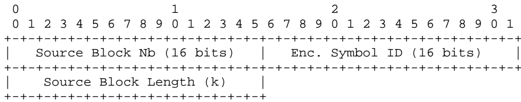
Figure 9: Repair FEC Payload ID encoding format for m = 16.
