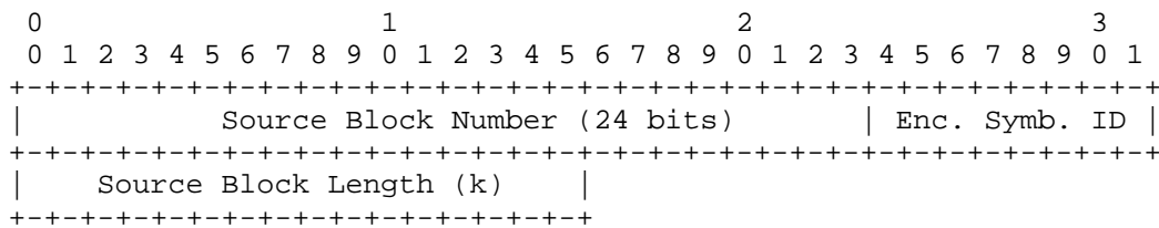
Figure 8: Repair FEC Payload ID encoding format for m = 8 (default).
