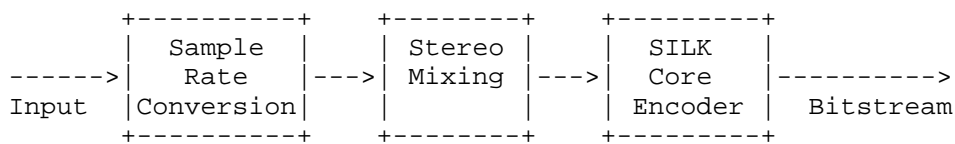
Figure 21: SILK Encoder
