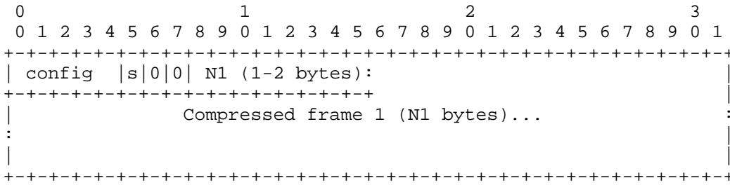
Figure 25: A Self-Delimited Code 0 Packet
