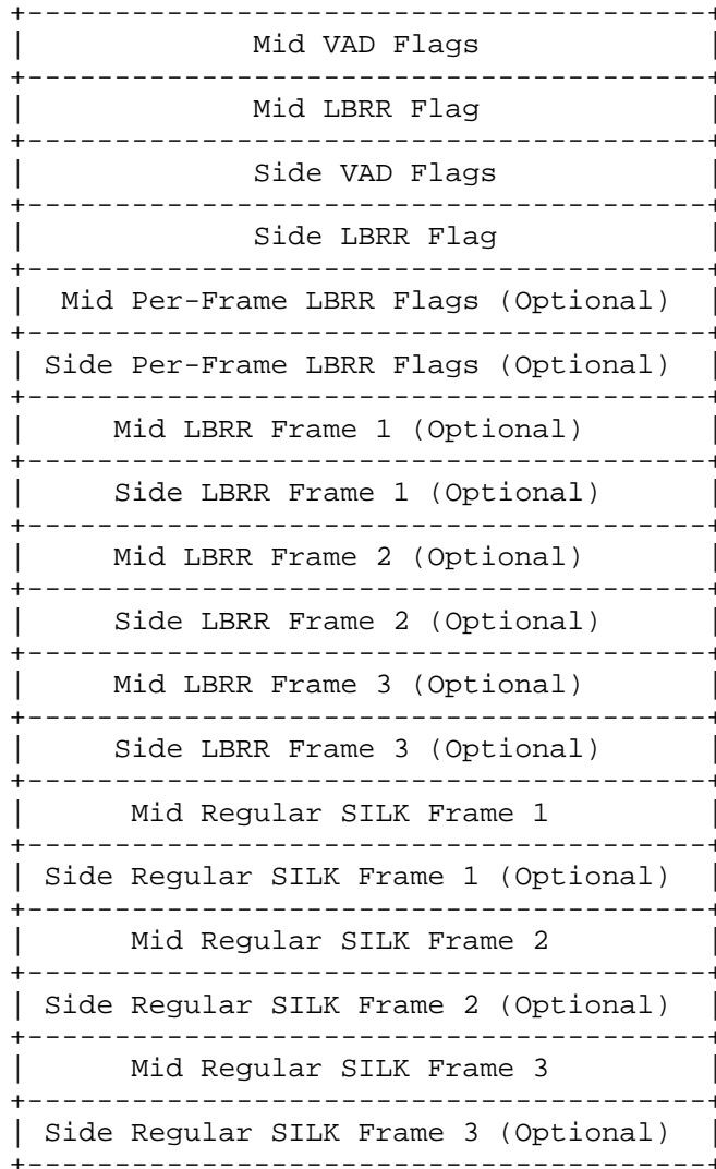
Figure 16: A 60 ms Stereo Frame
