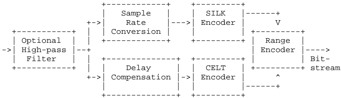
Figure 20: Opus Encoder
