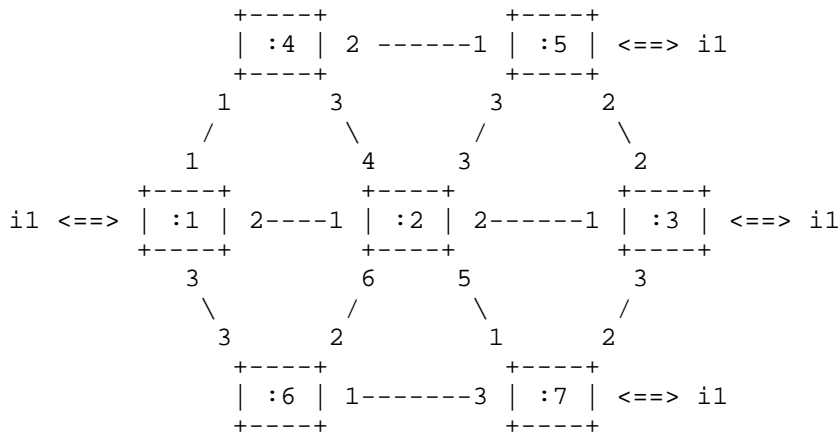
Figure 2: SPBM Example 7-Node Network
