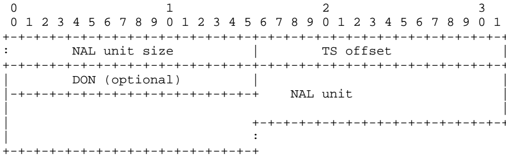
Figure 1. Non-interleaved multi-time aggregation unit for NI-MTAP
