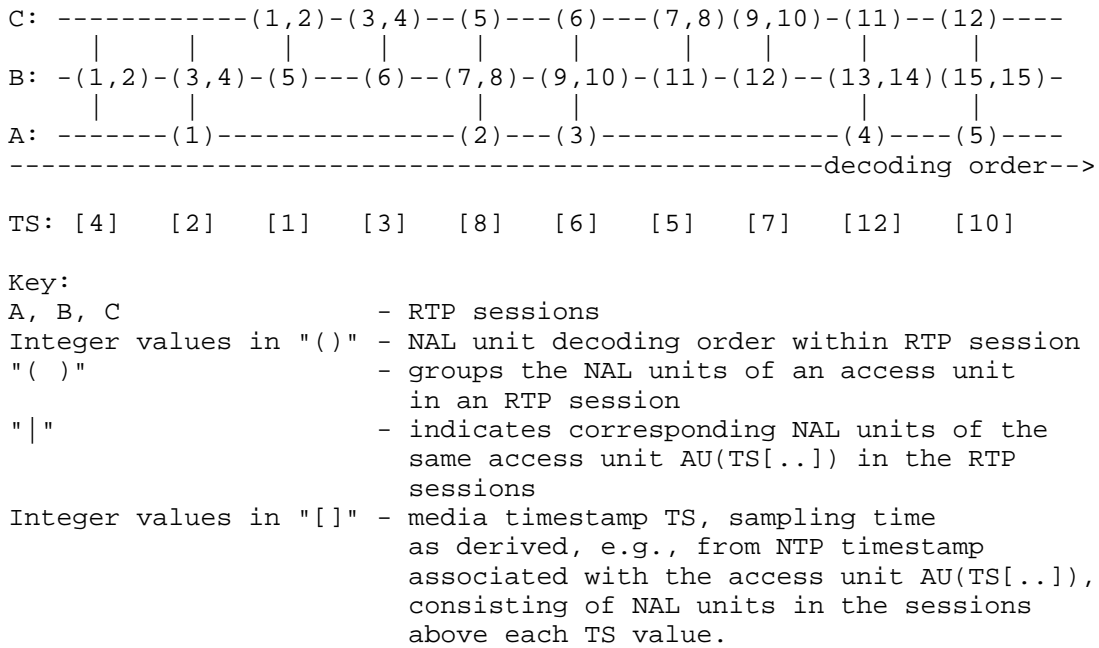
Figure 6. Example of decoding order recovery in multi-source transmission.
