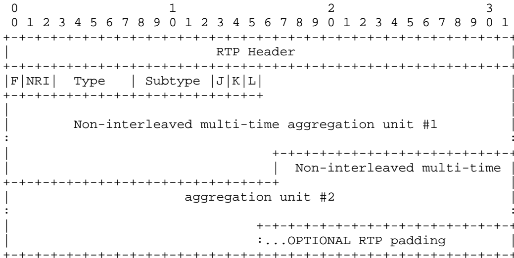
Figure 2. An RTP packet including an NI-MTAP containing two non-interleaved multi-time aggregation units
