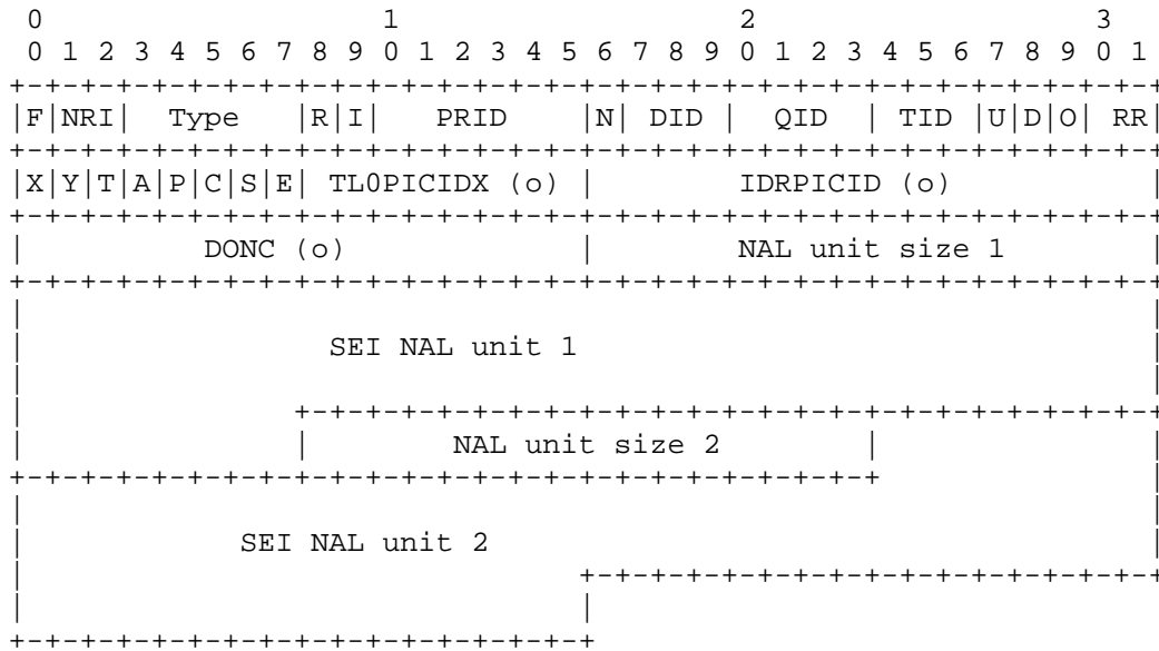
Figure 3. PACSI NAL unit structure. Fields suffixed by "(o)" are OPTIONAL.
