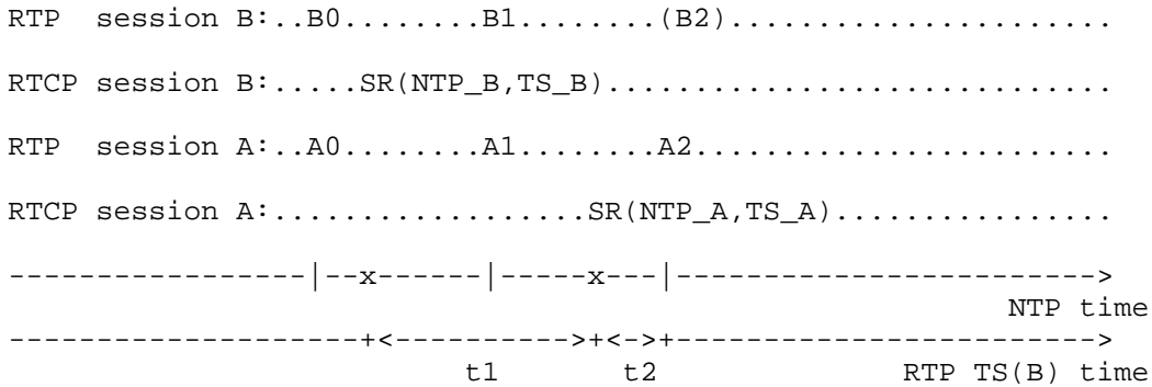
Figure 5. Example calculation of RTP timestamp for packet insertion in an enhancement layer RTP session
