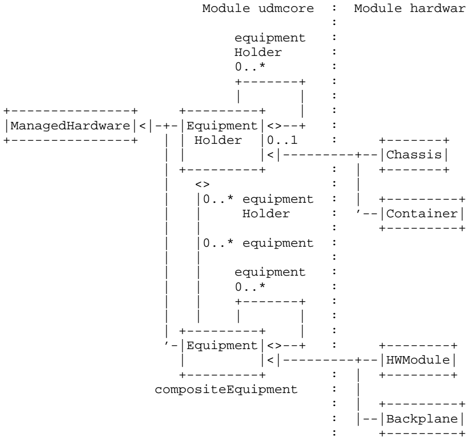
Figure 2: Hardware Entities Model
