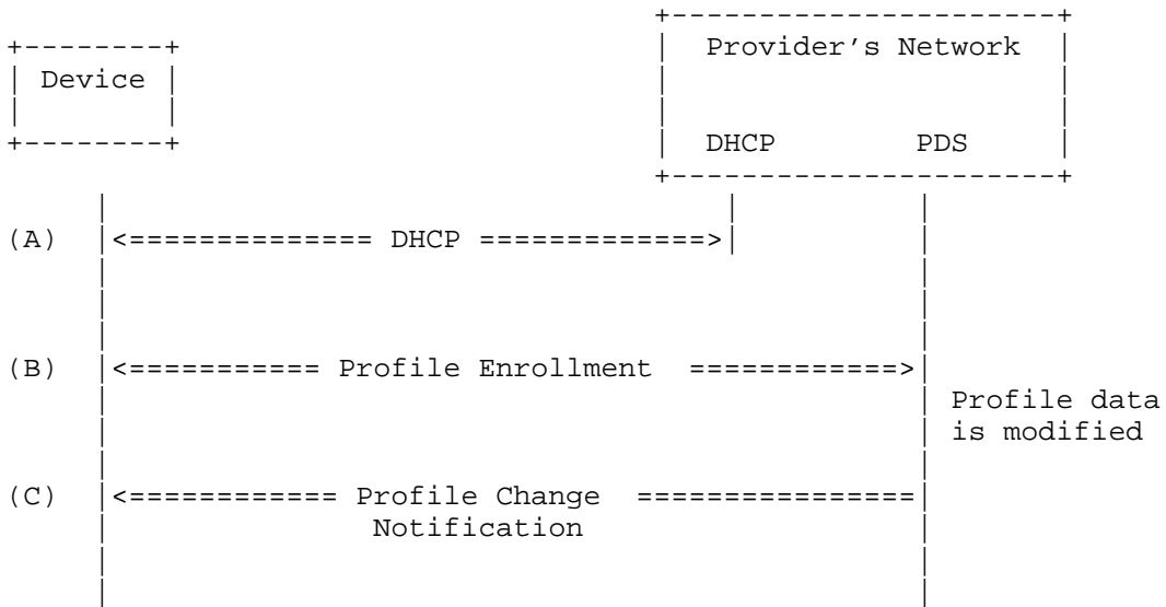
Figure 4: Use Case 1
